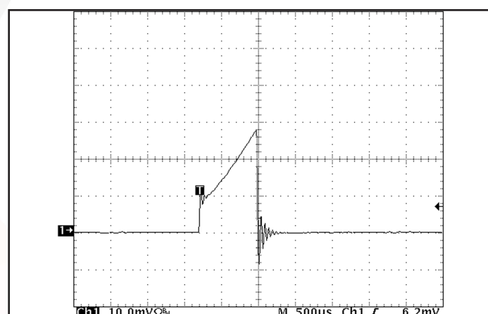
Figure 18: Load current (5A/div) as a function of time (500us/div) when the converter attempts to turn on into a 10 mΩ short circuit.
