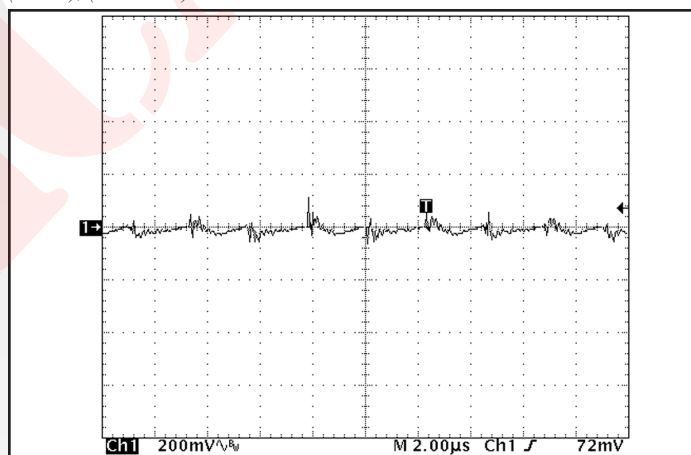
Figure 10: Output voltage ripple, 28Vout, at nominal input voltage and rated load current (200 mV/div), (2μs/div). Load capacitance: 1μF ceramic capacitor and 15μF tantalum capacitor. Bandwidth: 10 MHz. See Figure 17.
