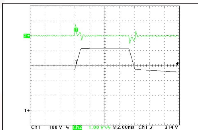
Figure 12: Output voltage response to step-change in input voltage (250V/ms). Load cap: 1μF ceramic and 15μF tantalum capacitors. CH 1: V_{in} (100V/div), CH 2: V_{out} (1V/div), (2ms/div).
