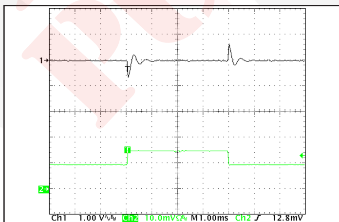
Figure 11: Output voltage response to step-change in load current (50%-75%-50% of I_{out(max)} ; dI/dt = 0.1 A/\mu s ). Load cap: 1 μF ceramic and 15 μF tantalum capacitors. CH 1: V_{out} (1V/div), CH 2: I_{out} (5A/div), (1ms/div).
