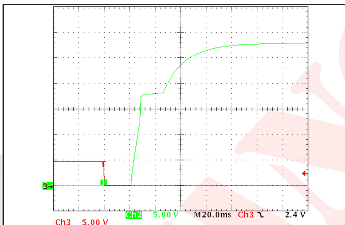
Figure 7: Typical startup waveform. Input voltage pre-applied, CH2: V_{out} (5V/div), CH3: ON/OFF (5V/div), Horizontal scale (20ms/div).
